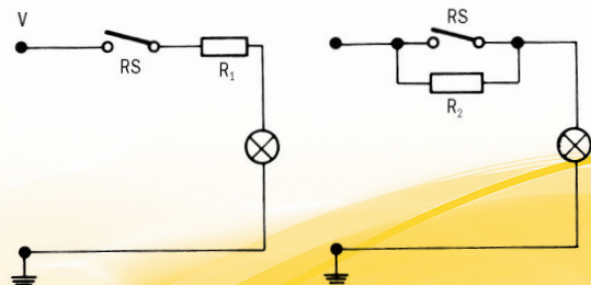
图5 Fig. 5 灯泡和电阻并联或者与转换开关串联的线路 Lamp load resistance in parallel or in series with switch.
