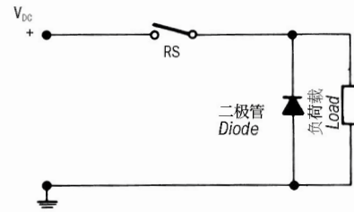
图1 Fig. 1 对于感应负载, 用半导体二极管做直流电防护 Direct current protection with semiconductor diode for inductive loads.
