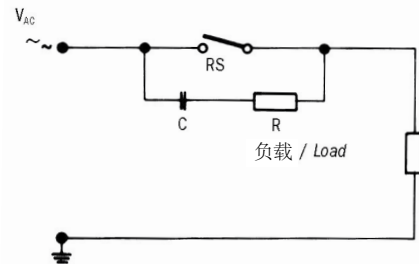
图2 Fig. 2 对于感应负载, 用RC连接方式做交流电防护 Alternating current protection with RC link for inductive load.
